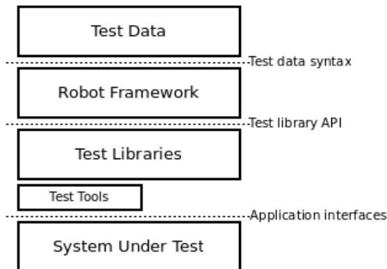
Figure 1: Robot Framework architecture
