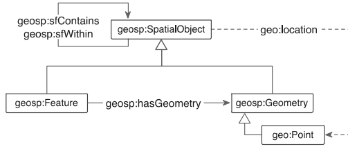
Figure 2: Topology model
