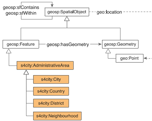
Figure 3: Administrative Area model
