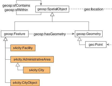
Figure 4: City Object model
