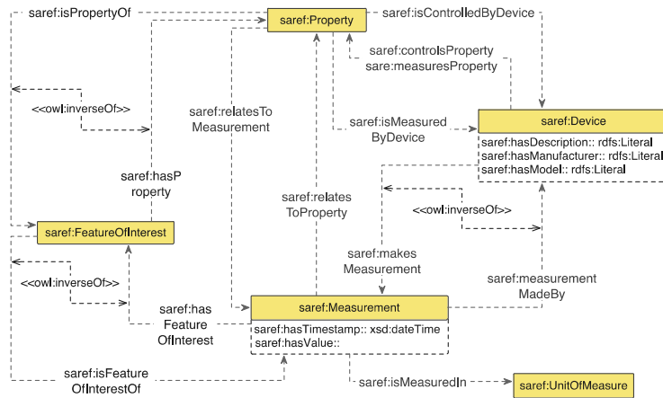
Figure 6: Measurement model
