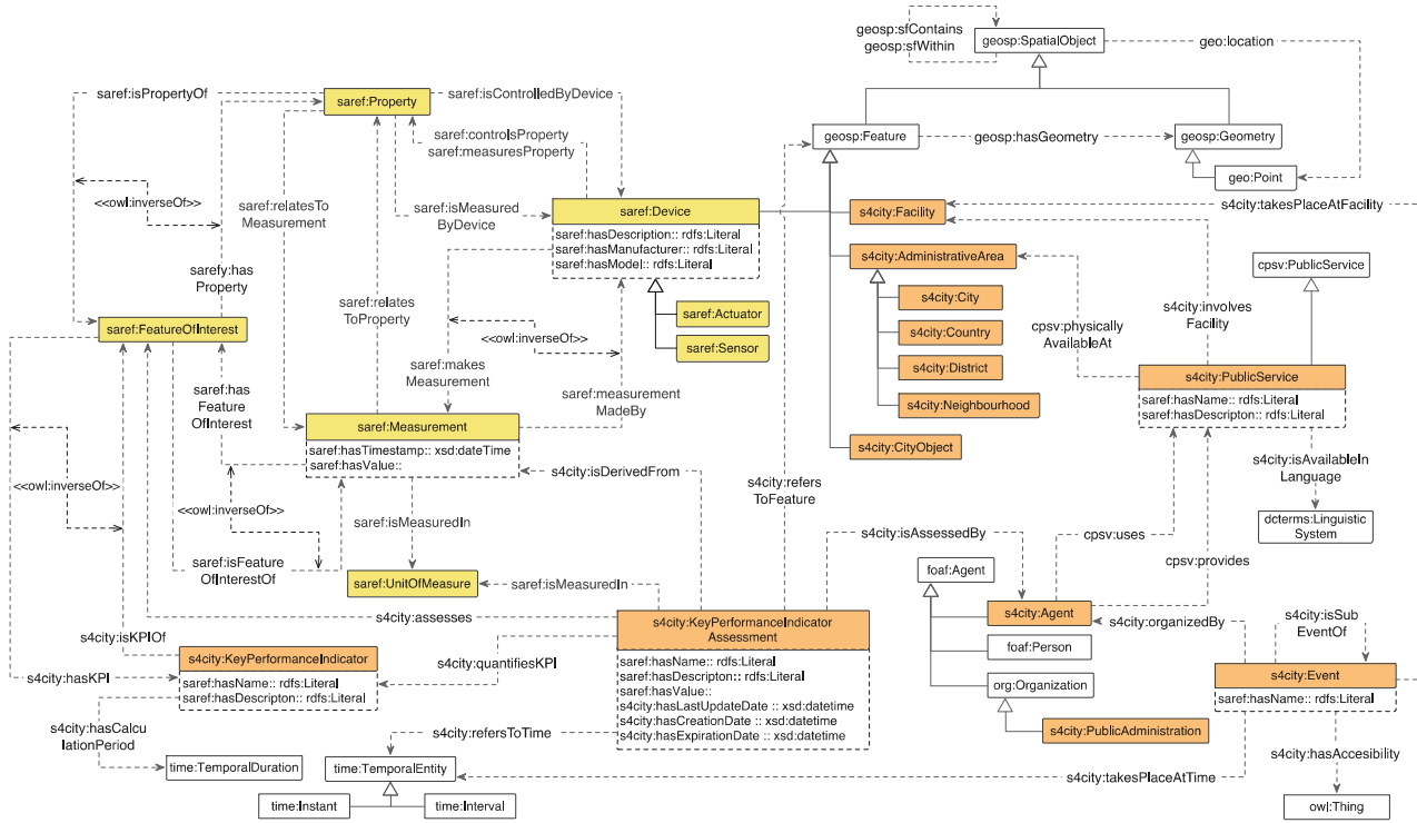
Figure 1: SAREF4CITY overview
