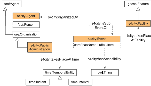
Figure 5: Event model
