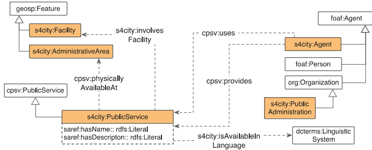
Figure 8: Public Service model
