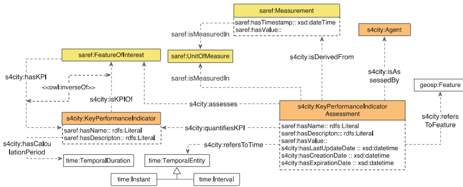
Figure 7: Key Performance Indicator model
